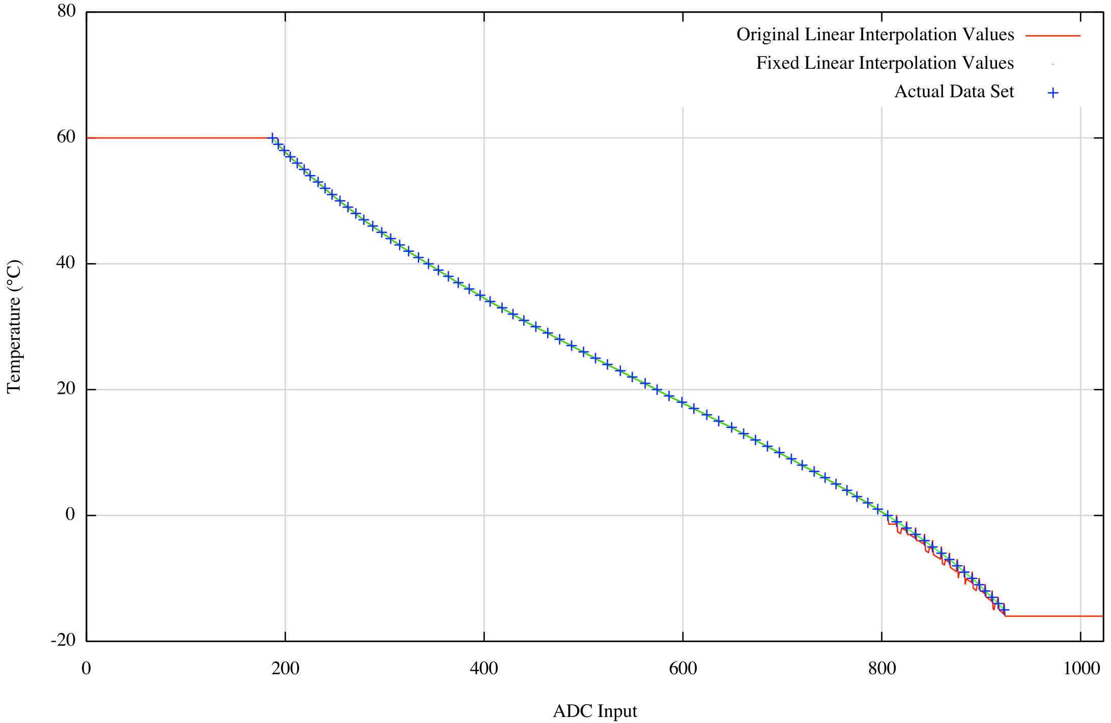
Verification of ADC2Temp Function
