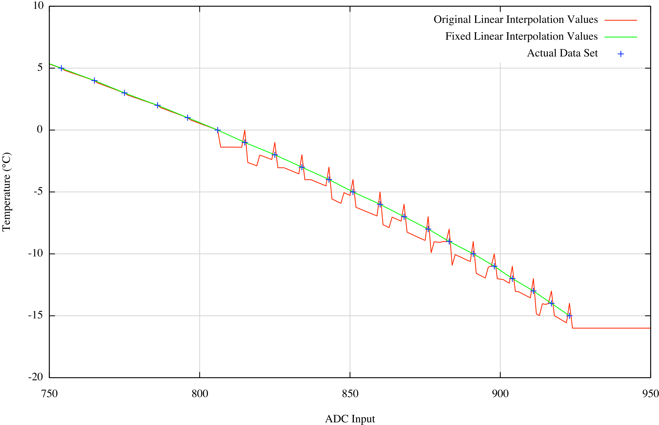
Verification of ADC2Temp Function (close-up)
